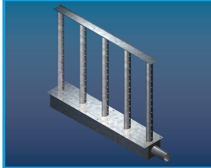
Multi-Steam™ HD High efficiency steam distributor (channel and header) with steam ejector eyelets
